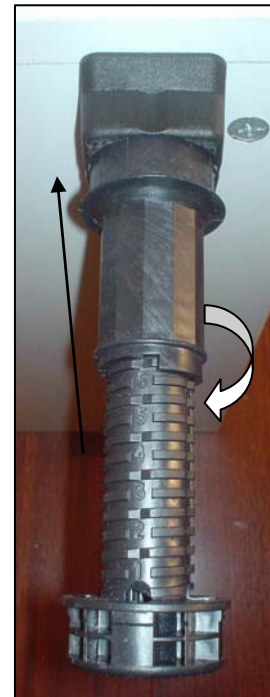
11.3 Fit Feet and Adjust Height
